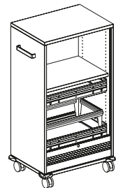
Height 1148 (3 binder height), width 600, depth 436 mm
